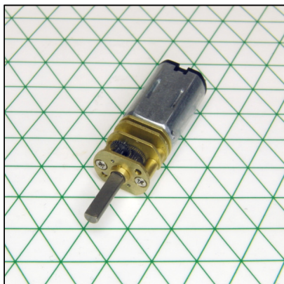
10mm DC Gearmotor - 24mm Type Shown on 6mm Isometric Grid
